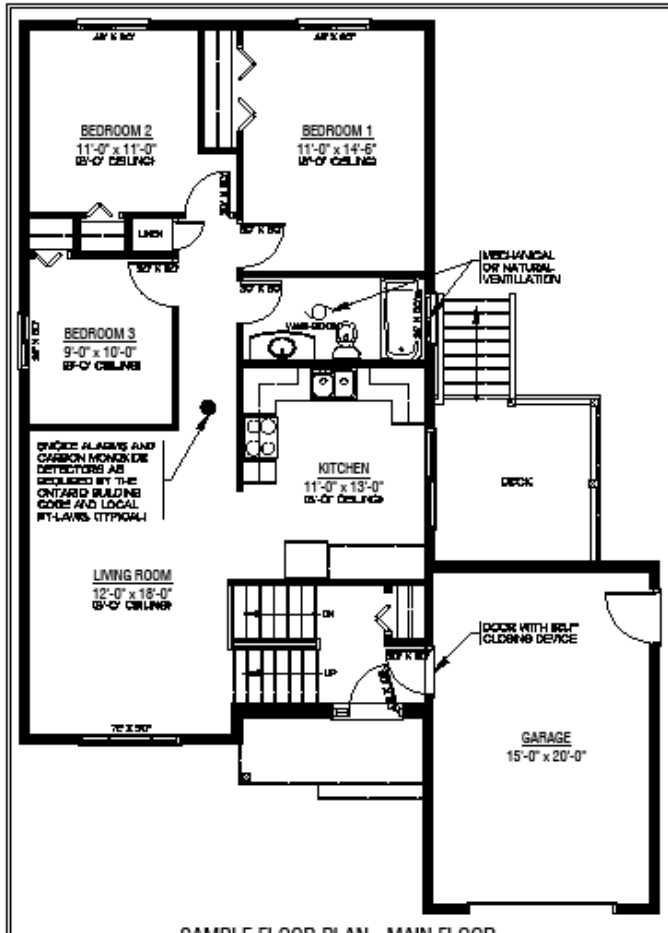
SAMPLE FLOOR PLAN - MAIN FLOOR
